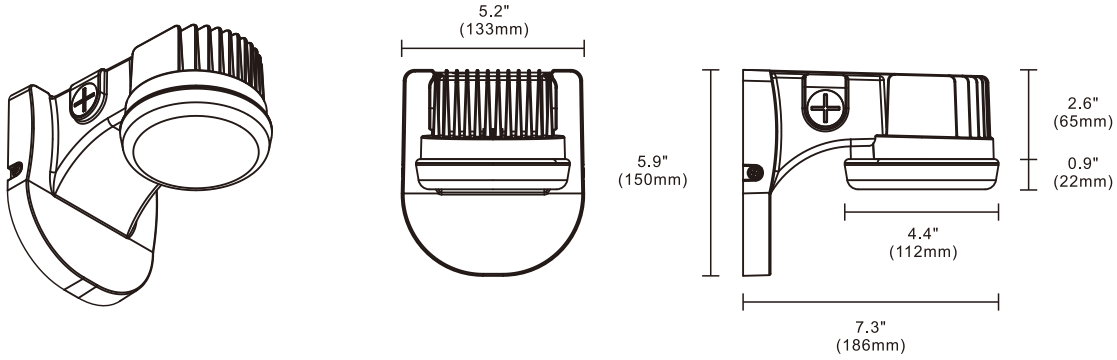
LED-1505C
