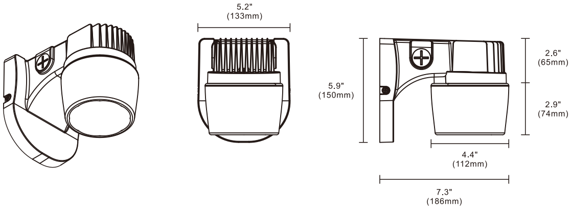
LED-1505CL
