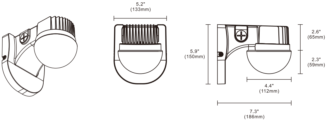
LED-1505B
